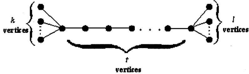
FIGURE 1: Binary star R(k, t, l) .
