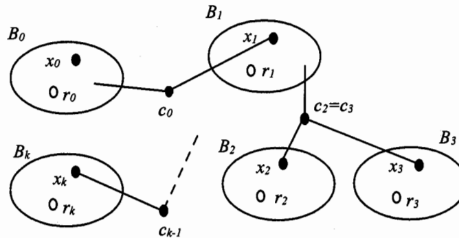
FIGURE 4: Algorithm diagram.
