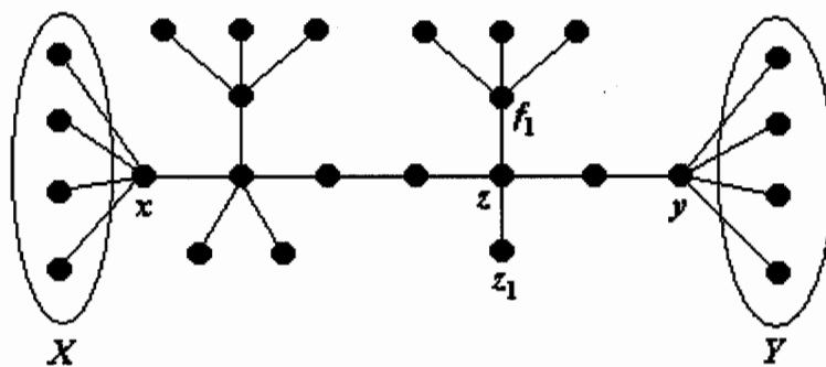
FIGURE 3a: A hypothetical graph G .
