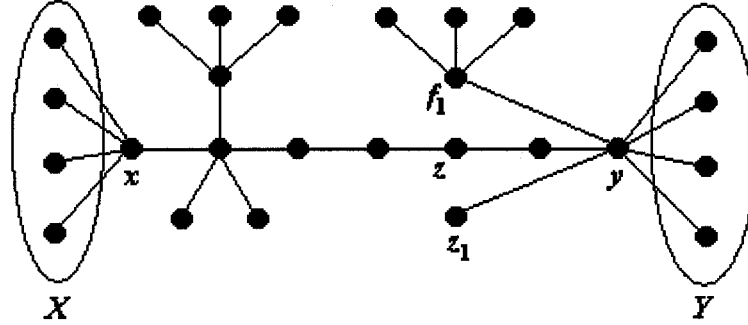
FIGURE 3b: The graph G' .
